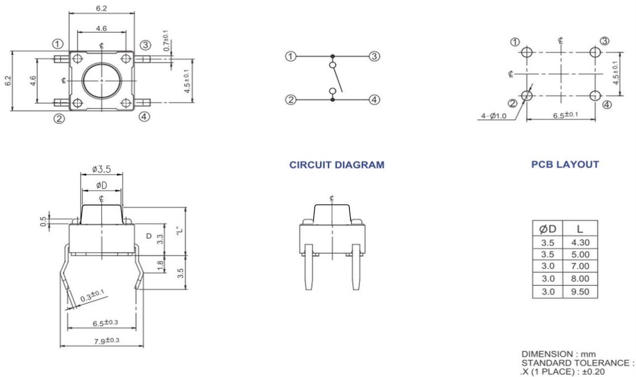
Figure 2 – Through-Hole, 222AD, Vertical Actuation
